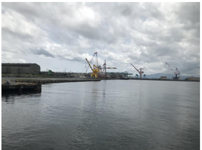
↑ Unloading PKS on the barge by yellow crane. Transport PKS by truck from here to the stockyard
